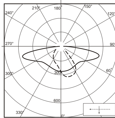
Wykresy KRS Light distribution diagrams cd/klm
