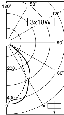
odbly nik prosty / flat louvre
